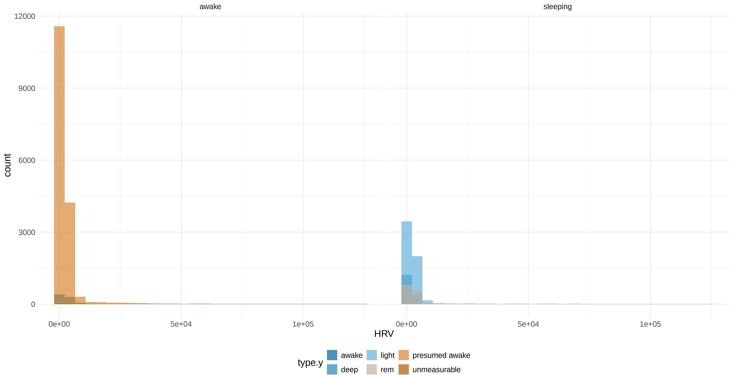
Histogram of HRV for FLARE011 split by waking and sleeping stages
